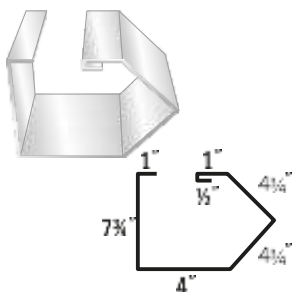
#55 Commercial Gutter
