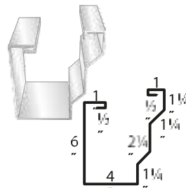
#53 Sculptured Gutter
