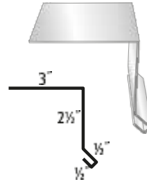
#44 Small Eave
