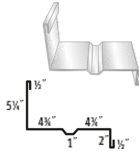
#23 One piece Fascia & Soffit
