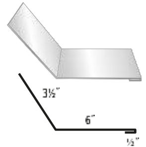
#15 Universal Endwall
