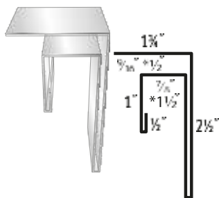
#16 "F" & "J" (AG) #17 "F" & "J" (*PBR)
