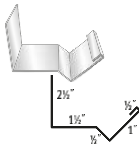
#38 Header Trim
