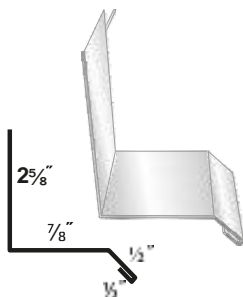
#12 Drip Cap (AG)
