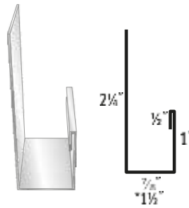
#8 "J" Trim (AG) #9 "J" Trim (*PBR)
