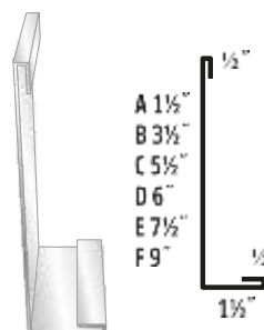
#14 Post Trim
