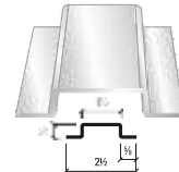
1/2" Sub Girt Length: 20'-0"
