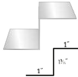
#48 Z Flashing
