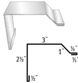
#24 Residential Rake
