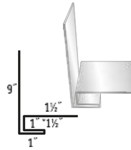
#19 Overhead Door Trim (AG) #20 Overhead Door Trim (*PBR)
