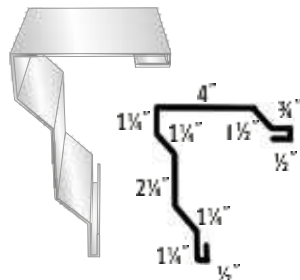
#32 Sculptured Rake
