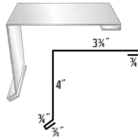
#49 Gable Rake Trim
