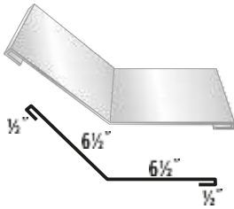
#67 Transition Flashing
