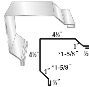
#3 Rake & Corner (AG) #78 Rake & Corner (*PBR)
