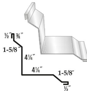
#18 Inside Corner
