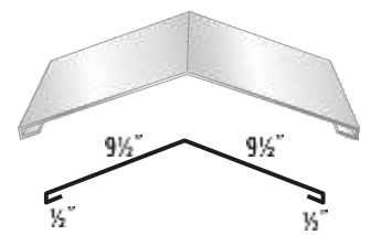
#40 XL Standard Ridge
