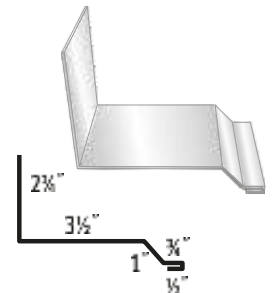
#11 Universal Sidewall
