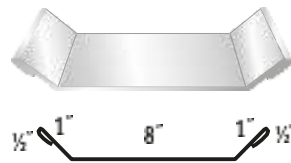
#77 Valley Cover
