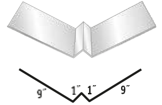
#25 Formed Valley
