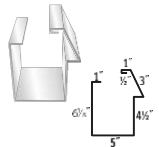
#54 Commercial Gutter
