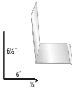
#28 'L' Flashing
