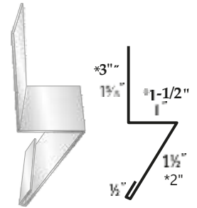
#4 Base Angle (AG) #5 Base Angle (*PBR)
