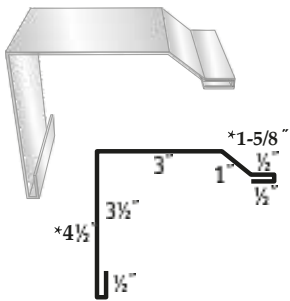
#31 Extended Rake (AG) #79 Extended Rake (*PBR)
