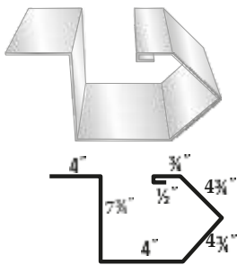
#51 LG Eave Gutter
