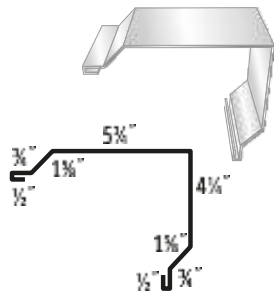
#7 Gable Trim
