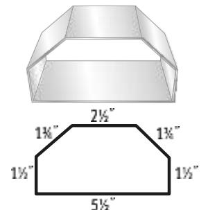
#65 Sculptured Downspout
