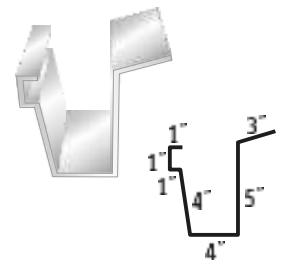
#50 Eave Gutter - Small
