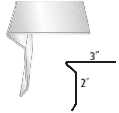
#45 Eave Trim
