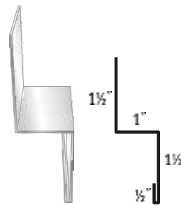
#10 Double Angle
