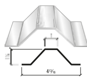
1-1/4" Hat Section Length: 12'-3"
