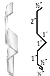
#34 Headwall Counter Flashing
