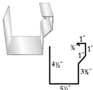
#56 Gutter
