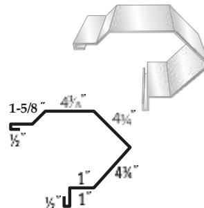
#33 Commercial Rake
