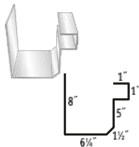
#52 Commercial Gutter
