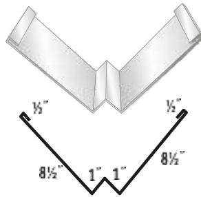
#42 SS Valley
