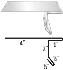
#22 'F' Trim
