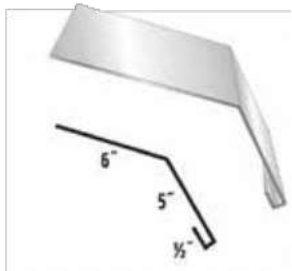
#27 Notched Gambrel
