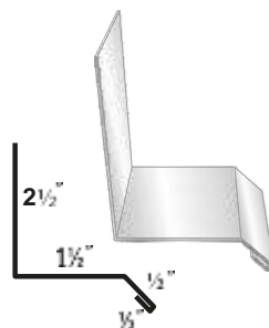
#13 Drip Cap (PBR)
