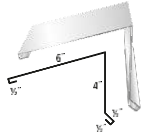
#80 Peak Cap
