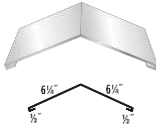
#2 (R) Standard Ridge Cap #2 (H) Standard Hip Cap
