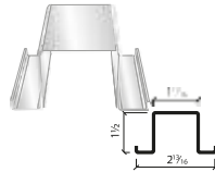
1-1/2" Hat Section Length: 20'-0"
