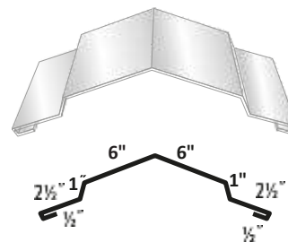
#39 XL Universal Ridge Cap
