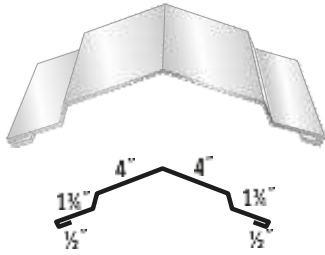
#1 (R) Universal Ridge Cap #1 (H) Universal Hip Cap
